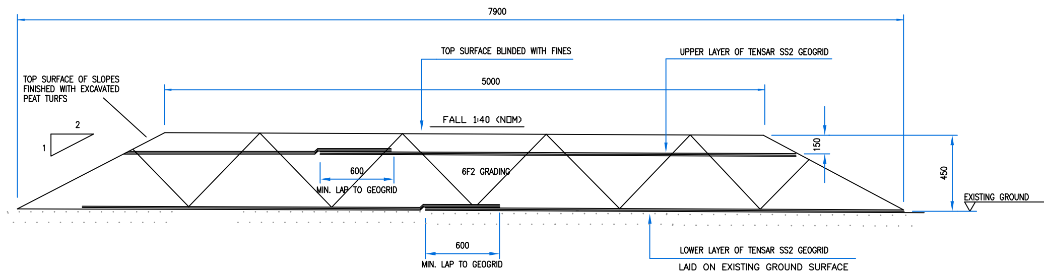
INDICATIVE SECTION OF ACCESS TRACK SCALE 1:40
