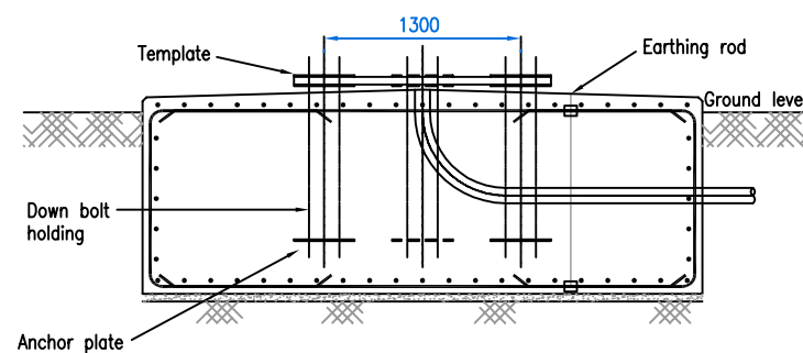
Section through mast foundation Scale 1:50
