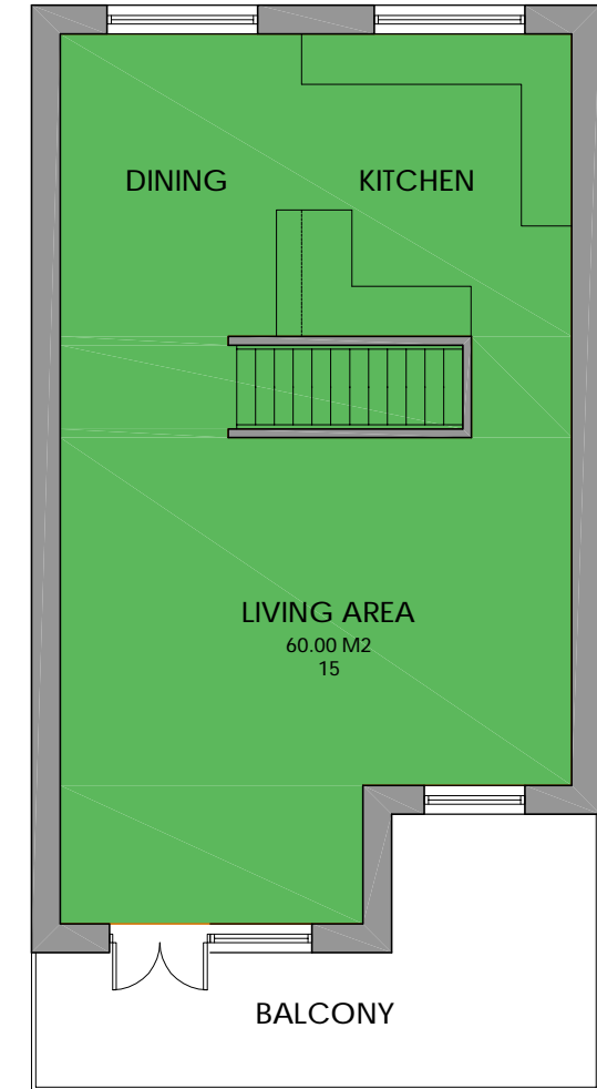
PROPOSED HOUSE TYPE B FIRST FLOOR 1:100 @ A3
