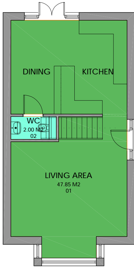
PROPOSED HOUSE TYPE A GROUND FLOOR 1:100 @ A3
